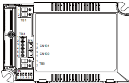
Terminal Pin No. Assignment(TB3)
