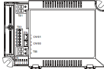
Terminal Pin No. Assignment(TB3)
