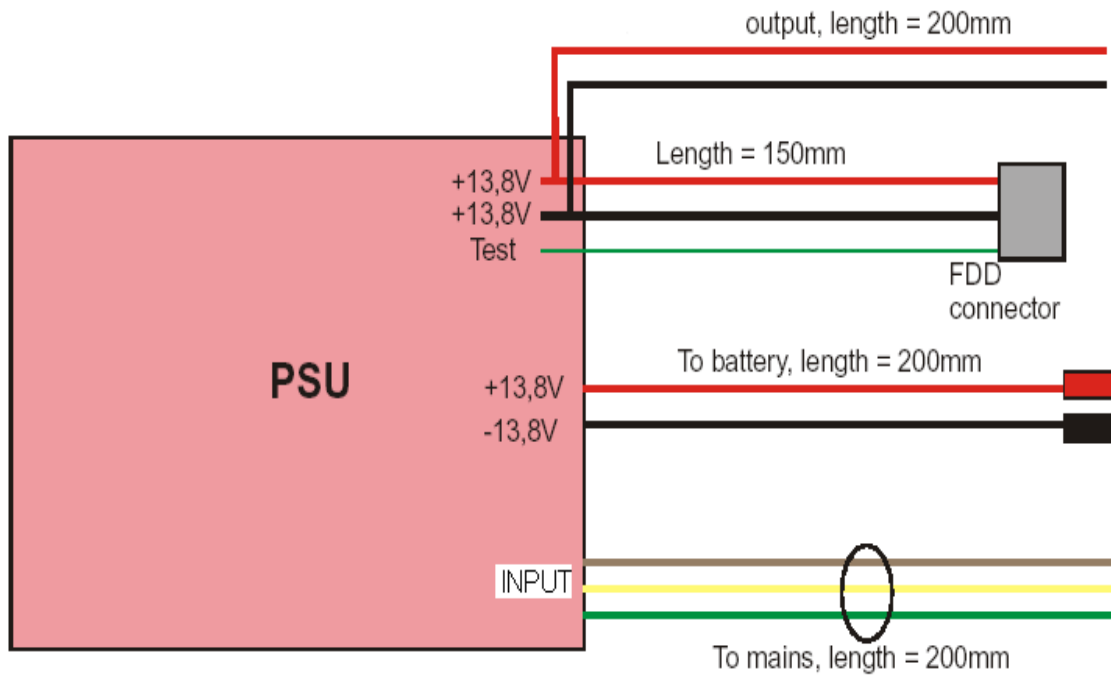
PSU external connections.
