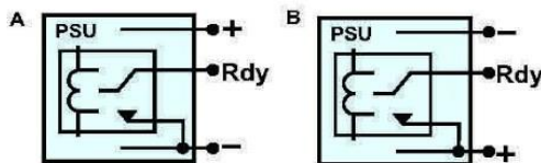
A: Rdy Internal Connection of T Type Terminal Block B: Rdy Internal Connection of E Type Terminal Block
