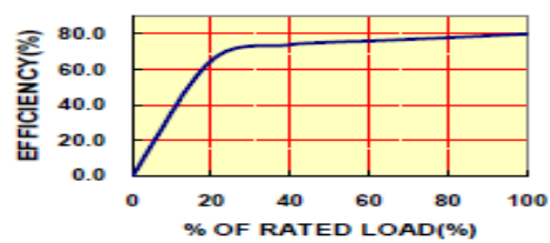
EFFICIENCY VS LOAD
